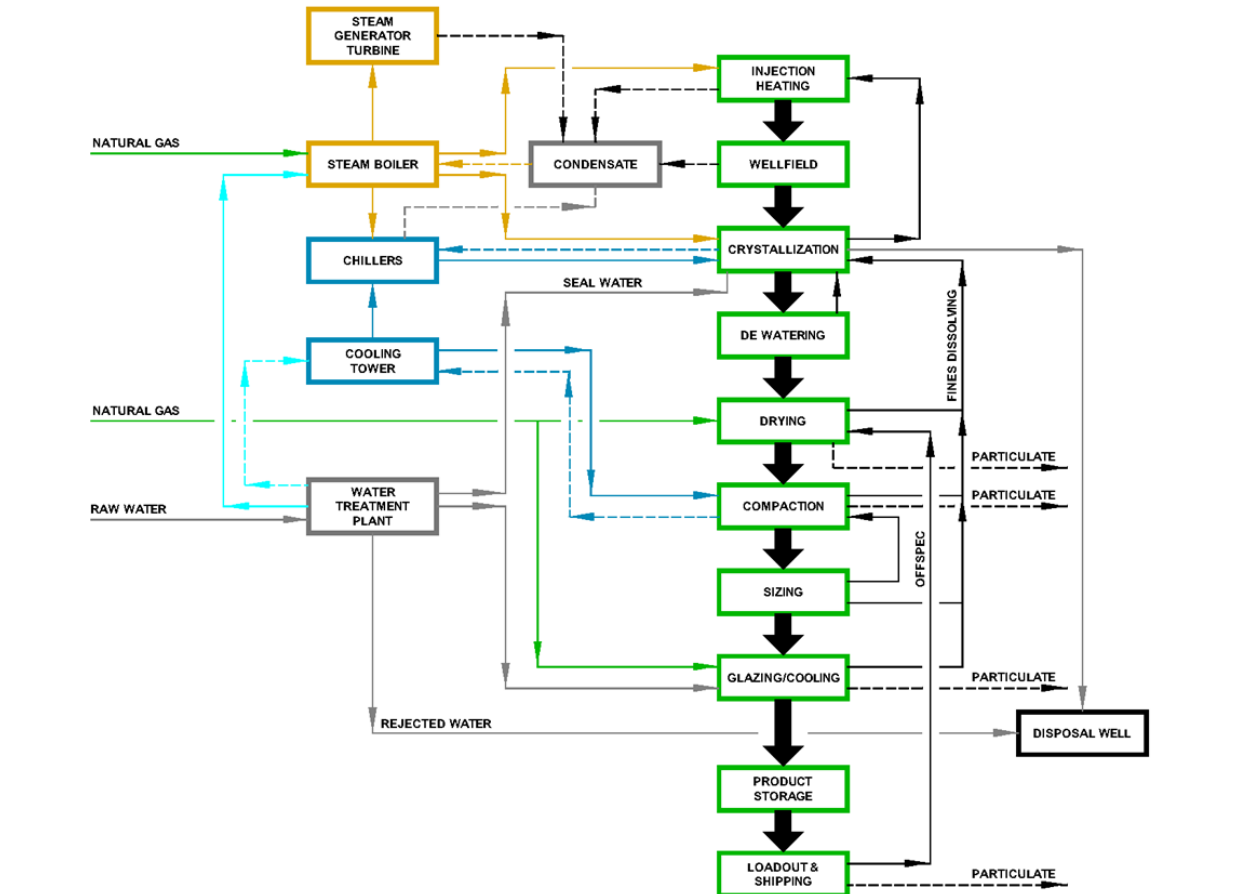
Figure 24: Simplified Process Block Diagram
